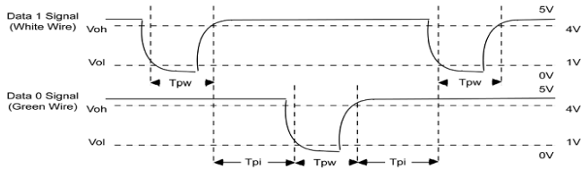
Figure 1 Sequence Diagram
